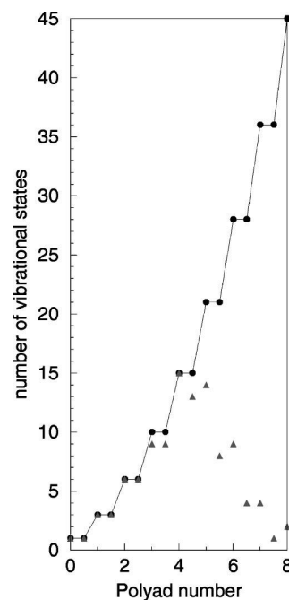
FIG. 1. Coverage of vibrational bands by polyad: possible (dots) and observed (triangles) vibrational bands in each polyad. The integer n on the x axis denotes the polyad n\nu and n+0.5 represents the polyad n\nu+\delta .
